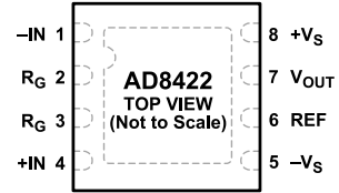
Figure 3. 8-Lead LFCSP Pin Configuration
