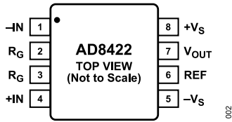
Figure 2. 8-Lead MSOP and 8-Lead SOIC_N Pin Configuration
