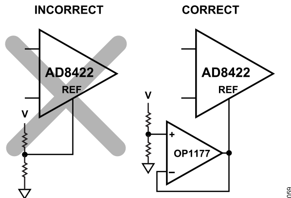
Figure 57. Driving the Reference Pin (REF)
