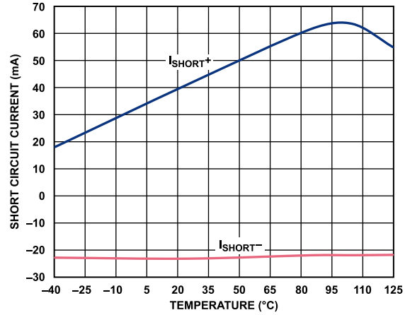
Figure 31. Short-Circuit Current vs. Temperature (G = 1)
