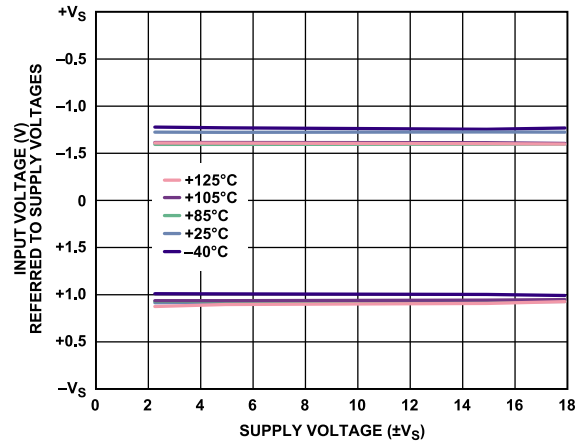
Figure 32. Input Voltage vs. Supply Voltage
